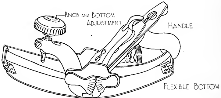
FIG. 65. CIRCULAR PLANE.
